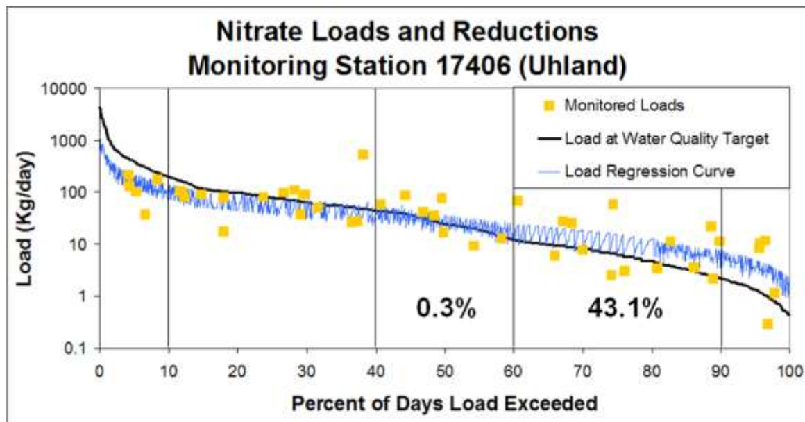
Figure 5.6. Nitrate load duration curve for station 17406 near Uhland in Hays County.
