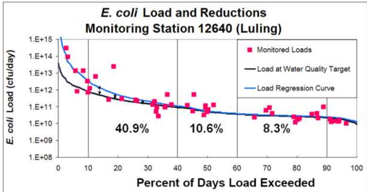
Figure 5.4. E. coli load duration curve for station 12640 near Luling in Caldwell County.
