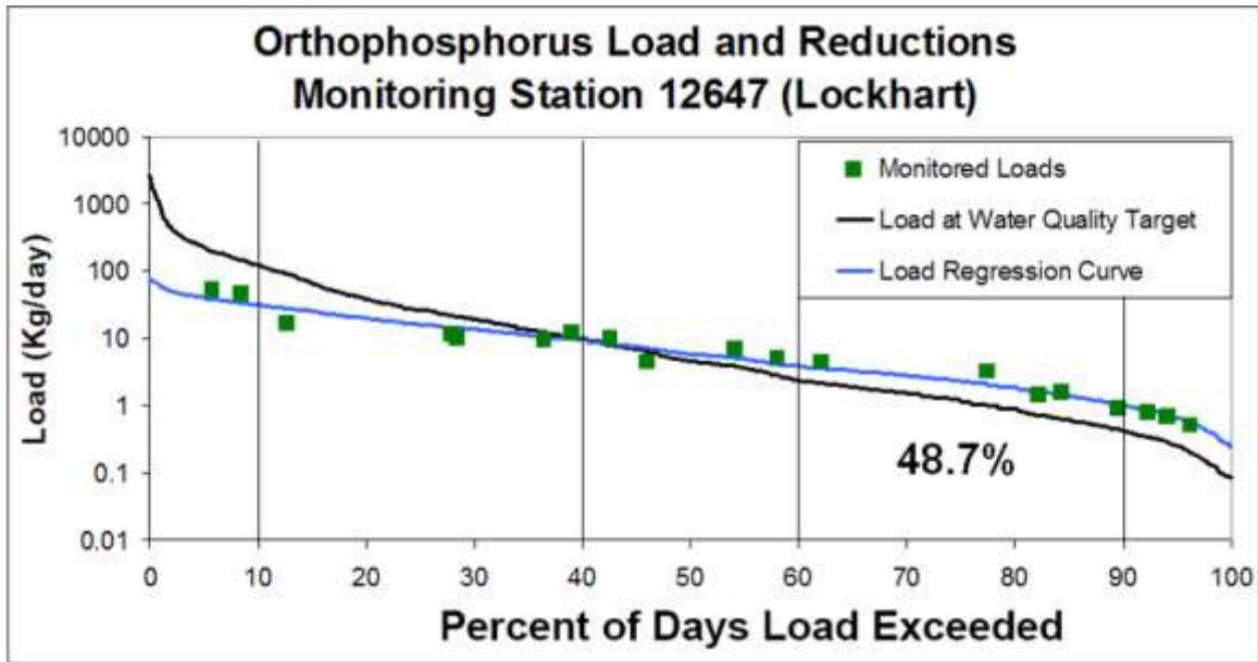
Figure 5.10. Orthophosphorus load duration curve for station 12647 near Lockhart in Caldwell County.
