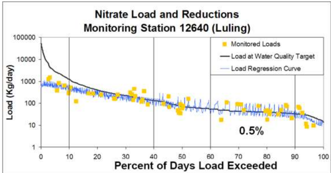
Figure 5.11. Nitrate load duration curve for station 12640 near Luling in Caldwell County.
