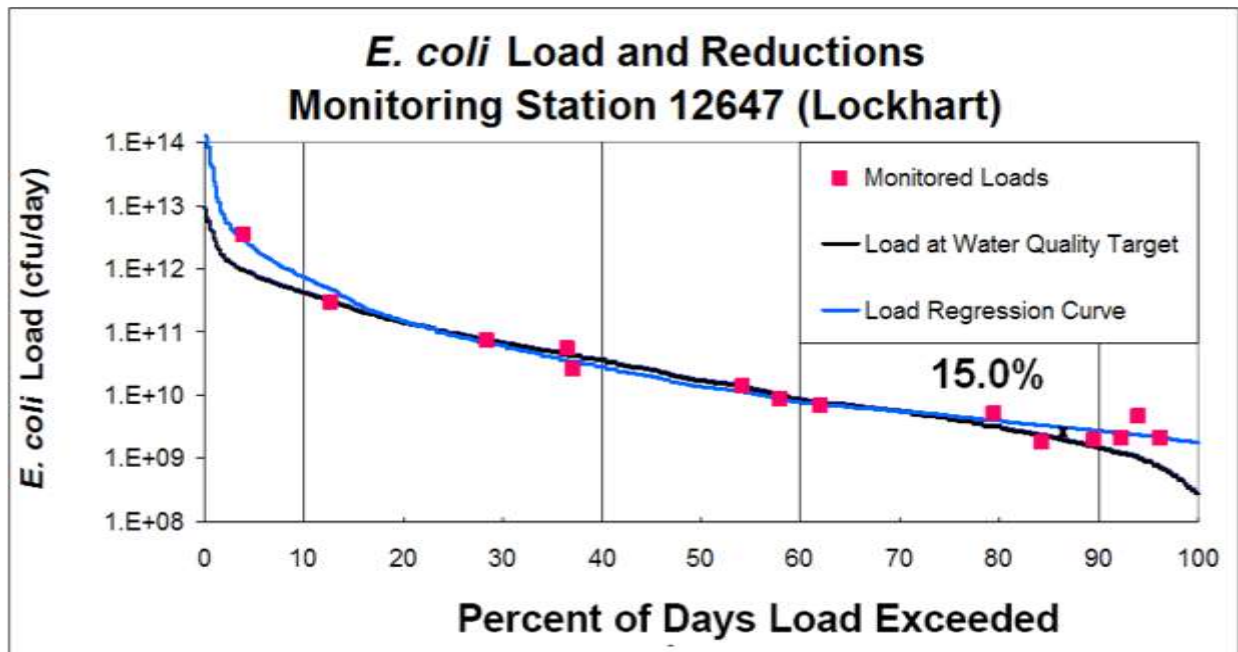
Figure E.4. Example load reduction for Lockhart monitoring station.
