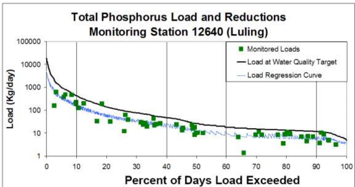
Figure 5.12. Total phosphorus load duration curve for station 12640 near Luling in Caldwell County.
