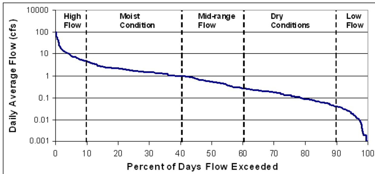
Figure E.1. Example flow duration curve. Vertical axis is flow rate and horizontal axis is percent exceedance. Curve shows percentage of time during a year, on average, a stream exhibits different flow conditions from very high flows during floods to low flow during summer or in long periods of time between rainfall events.
