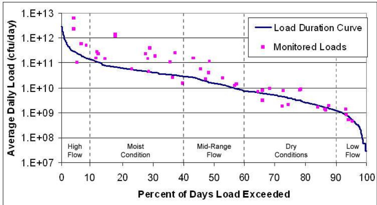
Figure E.2. Example load duration curve. Flow duration curve is multiplied by the E. coli bacteria criterion of 126cfu/100 mL to yield a maximum allowable bacterial load for a stream, varying with streamflow conditions.
