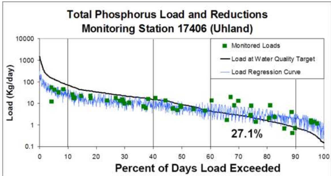
Figure 5.7. Total phosphorus load duration curve for station 17406 near Uhland in Hays County.
