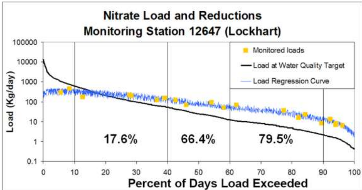
Figure 5.8. Nitrate load duration curve for station 12647 near Lockhart in Caldwell County.
