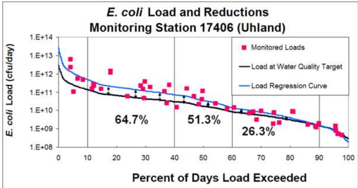
Figure E.3. Example load reduction determination for Uhland monitoring station.
