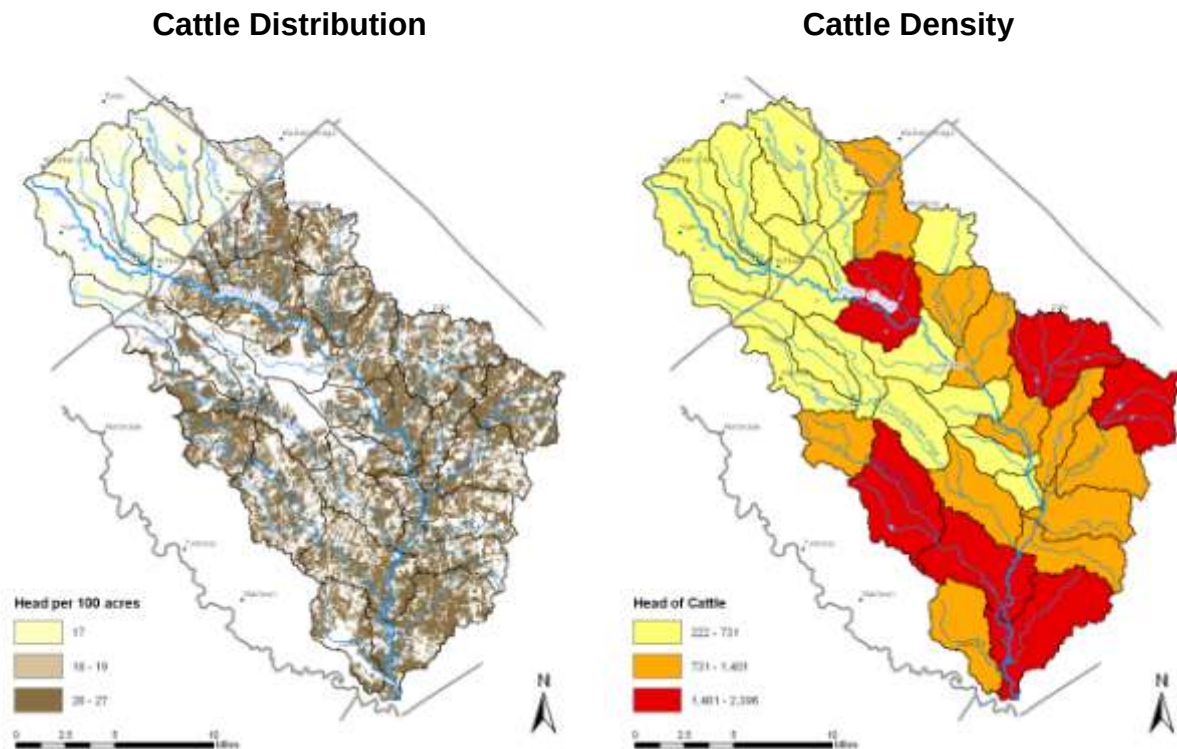
Figure F.6. Estimate cattle distribution and relative density in the Plum Creek Watershed.
